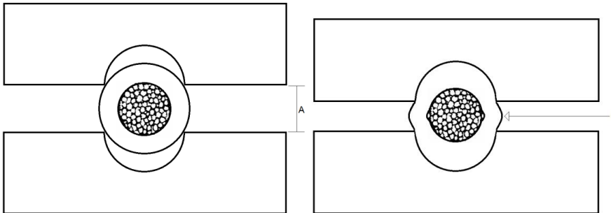
Figure 3: first contact between dies and fittings.
