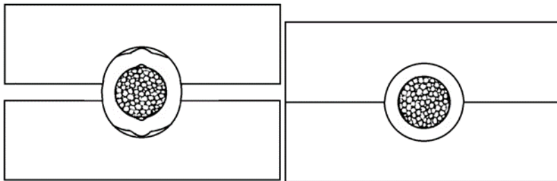
Figure 7: fitting has been rotated 90°. Dies have been closed to first contact fitting.
